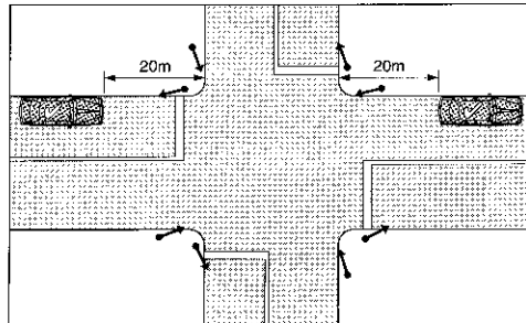
Example 1 Measurement of distance — intersection with traffic lights
